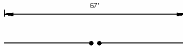
Fig. 1 7.15 MHz Dipole, #14 wire
